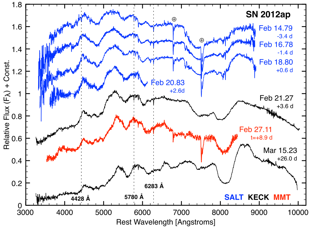
Figure 1. Optical spectra of the broad-lined Type Ic SN 2012ap during its first \sim 40 days after explosion. Three prominent DIBs around 4428 Å, 5780 Å, and 6283 Å are highlighted with dashed lines. SALT and Keck data have a 4–6 Å FWHM resolution. MMT data have 7 Å FWHM. Symbols show telluric absorptions in the SALT spectra that have not been corrected. Spectra have been corrected for a redshift of z = 0.0121 measured from narrow H II region lines of [O III] \lambda\lambda 4959, 5007, \text{H}\alpha , and [N II] \lambda\lambda 6548, 6583 observed near the location of the supernova.
