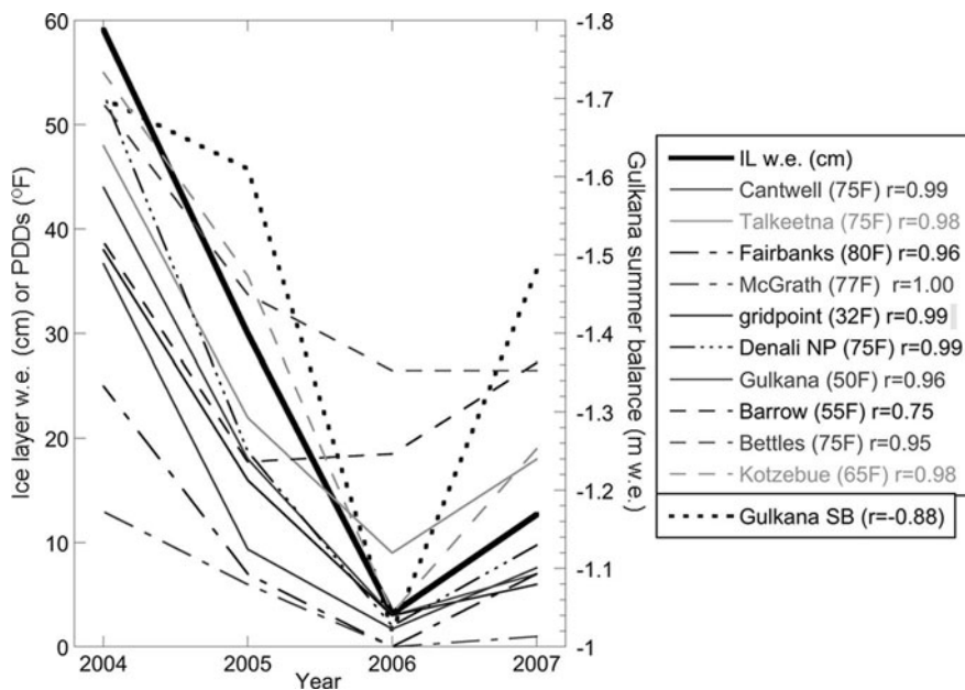
Fig. 3. Plot of annual firn-core ice-layer w.e. (thick solid line) or PDD above each station's respective threshold daily maximum temperature and Gulkana Glacier summer mass balance (dotted line, inverted right y-axis). Correlation coefficients between the ice layer w.e. thickness and the heat proxies are listed in the legend.
