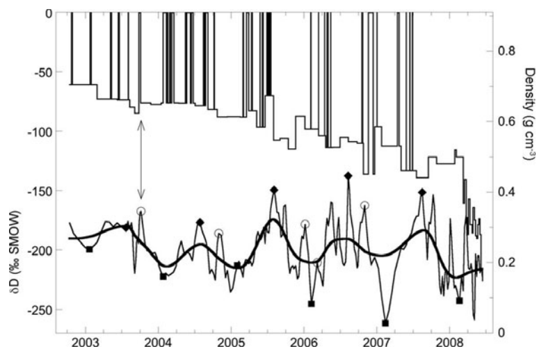
Fig. 2. Kahiltna Pass firn-core density (top), high-resolution \delta D (bottom, thin), smoothed \delta D (bottom, thick), peak summer markers (diamonds), peak winter markers (squares) and significant \delta D events (open circles) with a timescale as the x-axis. The arrows indicate the thickest ice layer (0.13 m) in the record and its associated spike in \delta D . The smoothed \delta D was done using a robust spline smoother (Meeker and others, 1995). The relative thickness of the density layers and their relative spacing do not correspond to their relative physical thickness and spacing because of linear interpolation between reference horizons with time as the independent variable.
