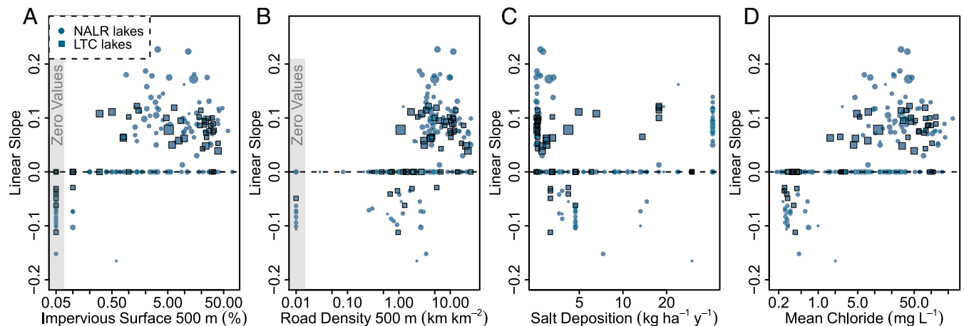
Fig. 3. Scatterplots of linear regression slope values versus (A) impervious surface within a 500-m buffer, (B) road density within a 500-m buffer, (C) rate of atmospheric salt deposition, and (D) mean in-lake chloride concentration over the entire time series for all NALR sites ( n = 284 ). In all plots, the size of the symbol is scaled by lake area. Squares with black borders denote LTC lakes. In A and B, zero values have been adjusted to fit on the x axis and are highlighted in gray.
