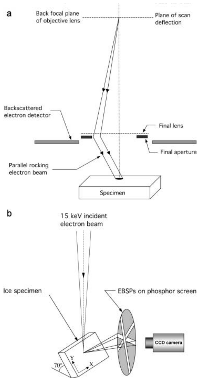
Fig. 2. Set-up for (a) SACP collection and (b) EBSP collection.
