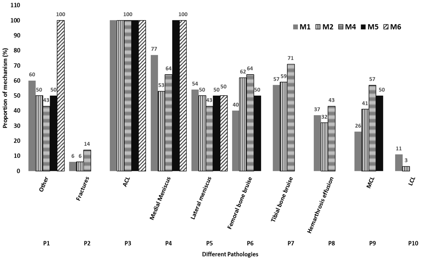
Fig. 1. Clustered bar chart of proportion (%) of each mechanism by pathology. There may be multiple pathology responses per mechanism. ACL, anterior cruciate ligament; LCL, lateral collateral ligament; MCL, medial collateral ligament.
