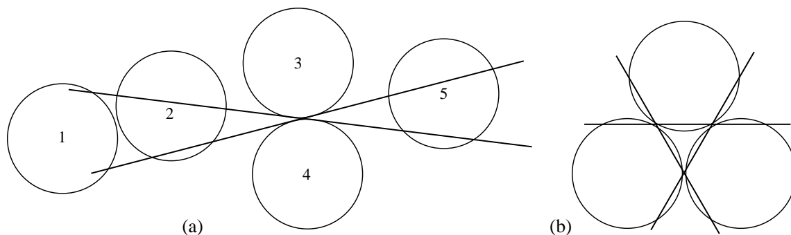
Figure 1: (a) Two line traversals with permutations (1, 2, 3, 4, 5) and (1, 2, 4, 3, 5) ; (b) Three permutations achievable.
