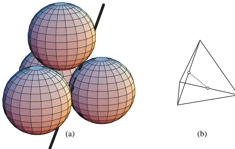
Figure 2: (a) A stabbing of three out of four congruent balls; (b) The centroids of the two pairs of unit-radius balls are separated by \sqrt{2} (dashed segment).
