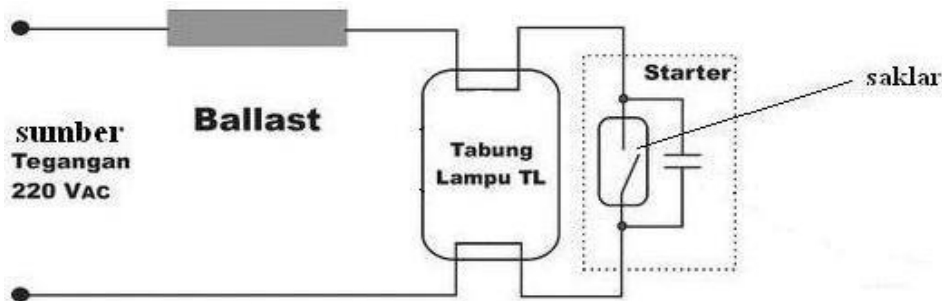
Gambar 2.3. Diagram lampu fluorescent
