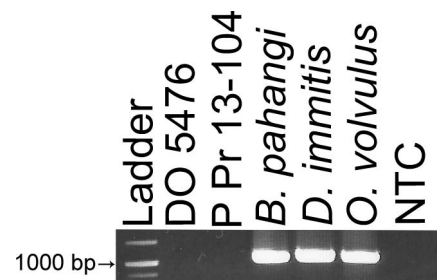
FIGURE 2. 16swolb PCR. Lane 1: 100-bp DNA ladder (New England Biolabs); Lane 2: DO 5476 ( Acanthocheilonema spirocauda ) genomic DNA; Lane 3: P Pr 13-104 ( A. spirocauda ) genomic DNA; Lane 4: Brugia pahangi genomic DNA; Lane 5: Dirofilaria immitis genomic DNA; Lane 6: DNA Onchocerca volvulus genomic DNA; Lane 7: no template control (NTC). Amplicons are at the expected size of 1,000 base pairs.
