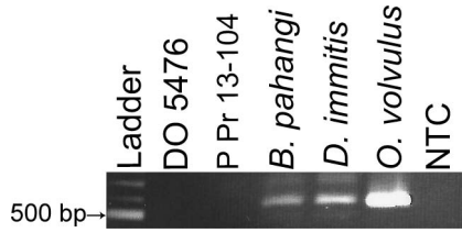
FIGURE 3. Wolbachia surface protein ( WSP ) PCR. Lane 1: 100-bp DNA ladder (New England Biolabs); Lane 2: DO 5476 ( Acanthocheiloneema spirocauda ) genomic DNA; Lane 3 P Pr 13-104 ( A. spirocauda ) genomic DNA; Lane 4: Brugia pahangi genomic DNA; Lane 5: Dirofilaria immitis genomic; Lane 6: DNA Onchocerca volvulus genomic DNA; Lane 7: no template control (NTC). Amplicons are of expected size of approximately 590 bp.
