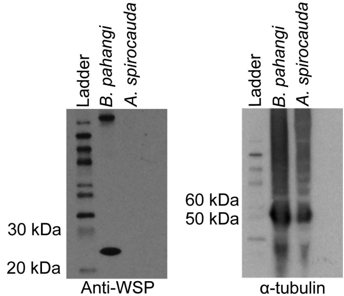
FIGURE 4. Left: Anti- Wolbachia surface protein ( WSP ) western blot. Left: Wolbachia surface protein appears between 20–30 kDa. Lane 1: Biotinylated ladder (Cell Signaling Technology no. 7727), Lane 2: positive control Brugia pahangi lysate, Lane 3: Acanthocheiloneema spirocauda lysate (DO-5476, whole worm). Right: Control western blot. Alpha-tubulin bands appear between 50–60 kDa. Lanes are the same as WSP blot.
