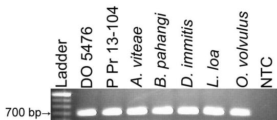
FIGURE 1. COI PCR for DNA quality verification. Lane 1: 100-bp ladder; Lane 2: DO 5476 ( Acanthocheilonema spirocauda ); Lane 3: P Pr 13-104 ( A. spirocauda ); Lane 4: Acanthocheilonema viteae ; Lane 5: Brugia pahangi ; Lane 6: Dirofilaria immitis ; Lane 7: Loa loa ; Lane 8: Onchocerca volvulus ; Lane 9: no template control (NTC).
