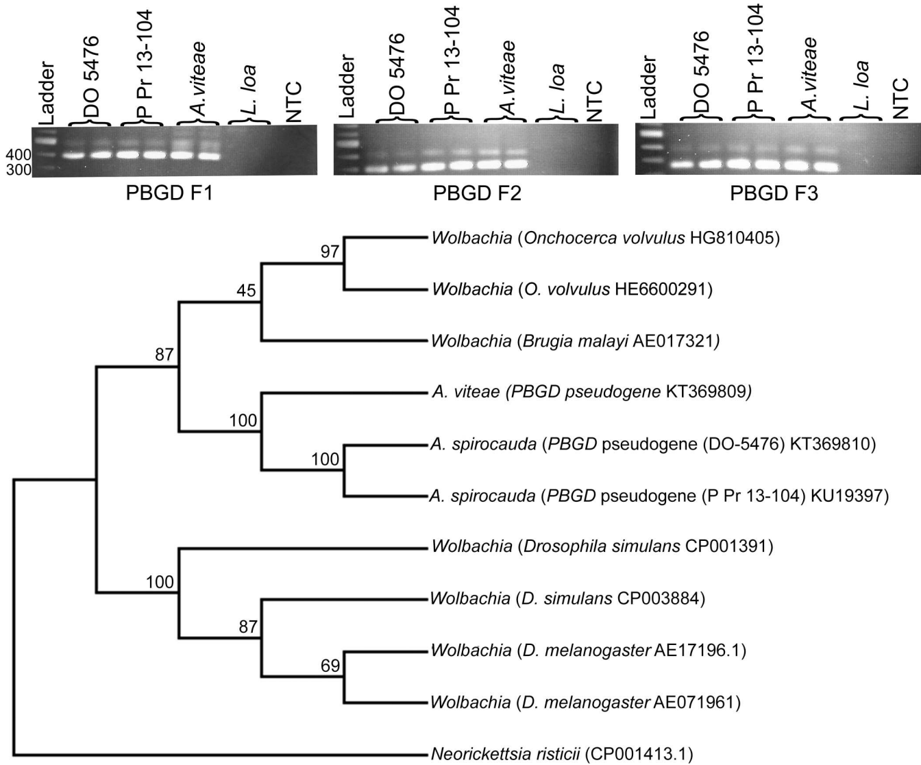
FIGURE 5. Top: porphobilinogen deaminase pseudogene ( PBGD ) gel images: Lane 1: 100-bp ladder (New England Biolabs); Lanes 2 and 3: Acanthocheilonema spirocauda genomic DNA (DO-5476); Lanes 4 and 5: A. spirocauda genomic DNA (P Pr 13-104); Lanes 6 and 7: Acanthocheilonema viteae genomic DNA; Lanes 8 and 9: Loa loa genomic DNA (negative control); Lanes 10 and 11: no template control. Bottom: Phylogeny of hemC ( PBGD ) pseudogene sequences. Bootstrap confidence values after 500 iterations are displayed at the nodes. Displayed are the PBGD sequences obtained in this study compared against the top 3 filarial parasite results indicated by BLASTn analysis as well as several insect Wolbachia sequences that showed similarity to the query sequence in BLAST.
