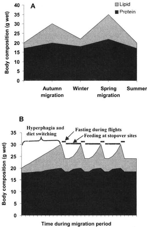
FIGURE 1. Change in body composition associated with migratory and nonmigratory periods of the annual cycle in a typical temperate-zone migratory songbird. (A) Body mass increases from approximately 20 g to 35 g between nonmigratory and migratory periods, and this increase in body mass is composed of primarily lipid and some protein stores. (B) In preparation for migration, birds accumulate fat stores primarily by increasing food intake and by carefully selecting their diets. Then during a given migration period, a typical migratory bird traveling between wintering and breeding areas must take several flights that are interspersed with layovers at stopover sites where the bird refuels in preparation for the next flight. Thus, birds during migration alternate between periods of high feeding rate at migratory stopover sites and periods without feeding as they travel between stopover sites.
