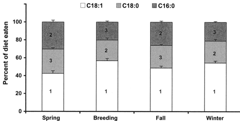
FIGURE 2. Percent ( \pm SE) of total food intake of Red-eyed Vireos ( n = 18 birds trial -1 ) during each three-way preference trial given at four different times of the year. The three diets were 41% carbohydrate, 13% protein, and 30% fat, but the fatty acid composition of the dietary fat in each diet was unique (>90% 16-carbon saturated [16:0], or 18-carbon unsaturated with one [18:1] or two [18:2] double bonds) because we used purified triglycerides. Vireos ate significantly more of the 18:1 diet compared to the 18:0 and 16:0 diets in all seasons ( P < 0.02 ). Numbers within the bars denote the rank order of preference based on compositional analysis.
