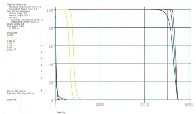
Gambar 3. Dose Volume Histogram (DVH)
