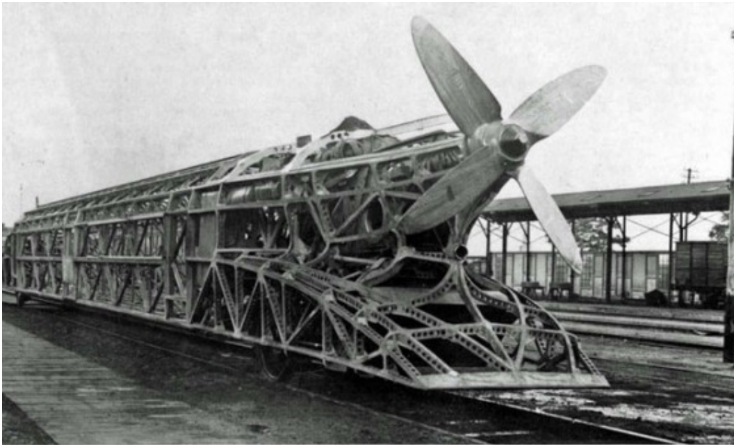
Rail Zeppelin of F. Krukenberg.
