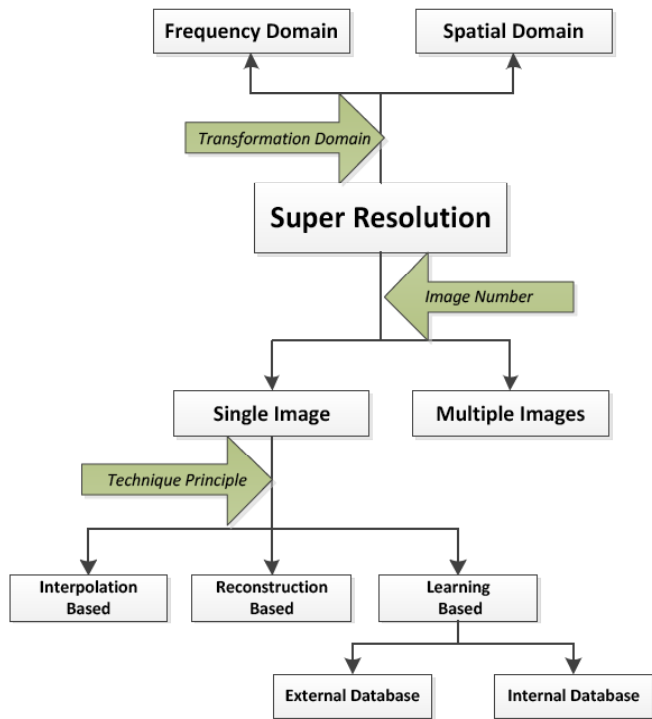
Figure 1: The taxonomy for super resolution algorithms.
