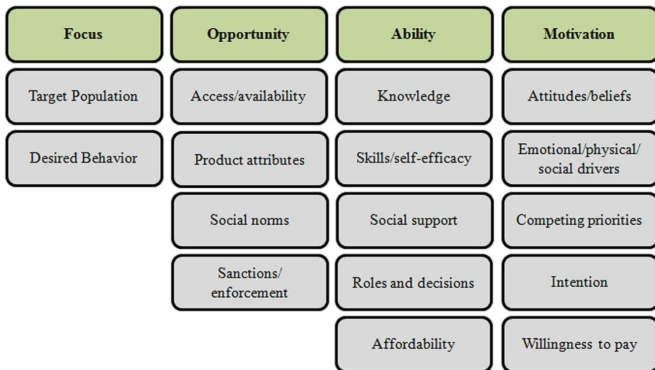
Figure 1. SaniFOAM Framework [14].
