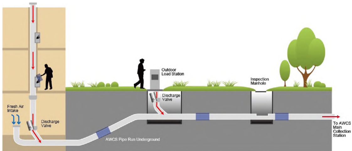
Figure 1 – Central system for solid waste collection
