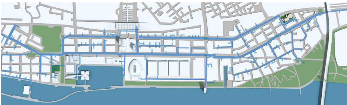
Figure 5 - Network of distribution of cold and heat of the Parque das Nações (ENGIE, 2017)
