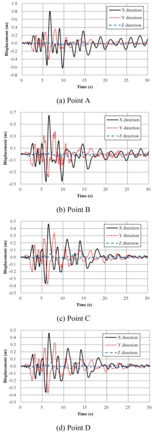
Figure 20. Seismic response behaviour (JR Takatori, Unfixed post condition \mu_s=0.3 , Limit strength calculation 1.5)
