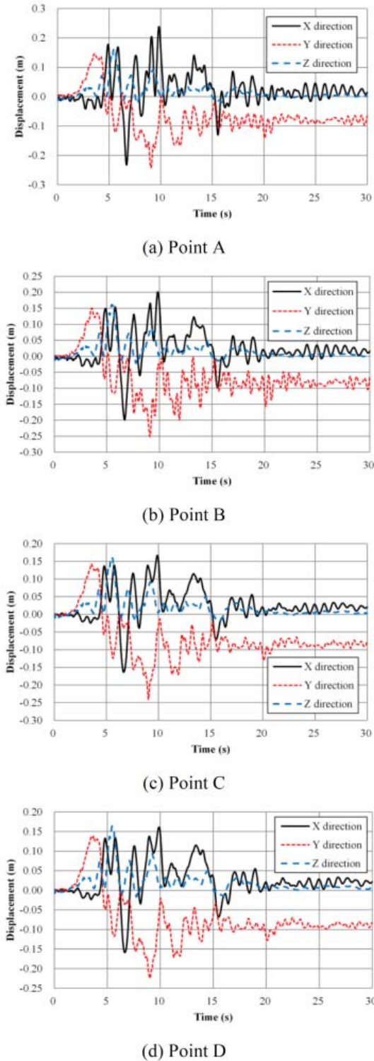
Figure 19. Seismic response behaviour (JMA Kobe, Unfixed post condition \mu_s=0.3 , Limit strength calculation 1.0)
