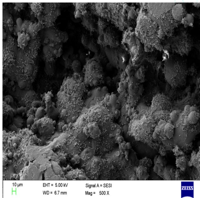
Fig.5) SEM Images at 500X magnification of precinol ATO 5 (wax) coated tablet surface.
