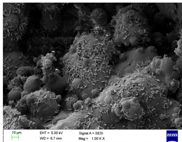
Fig.6) SEM Images at 500X magnification of precinol ATO 5 (wax) coated tablet surface.
