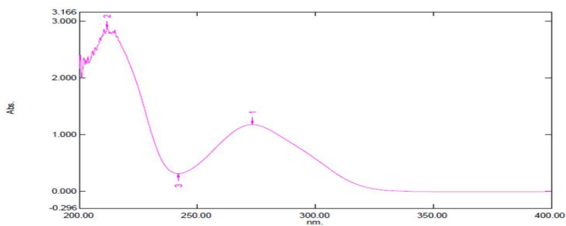
Figure 1.1 UV Spectrum of Gallic acid
