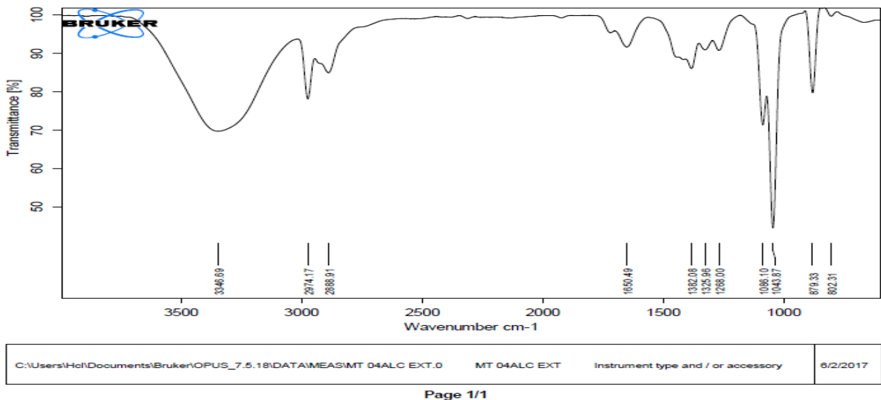
Fig. 2.6 FTIR spectrum of methanolic extract
