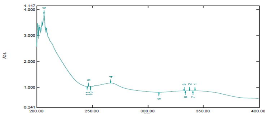
Fig. 1.6 UV spectrum methanolic extract
