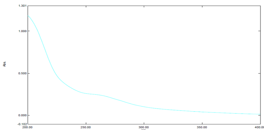
Fig. 1.7 UV spectrum aqueous extract
