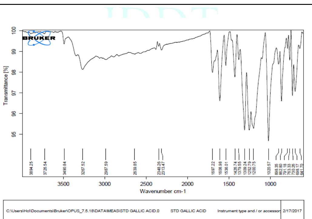
Fig. 2.1 FTIR spectrum of standard gallic acid
