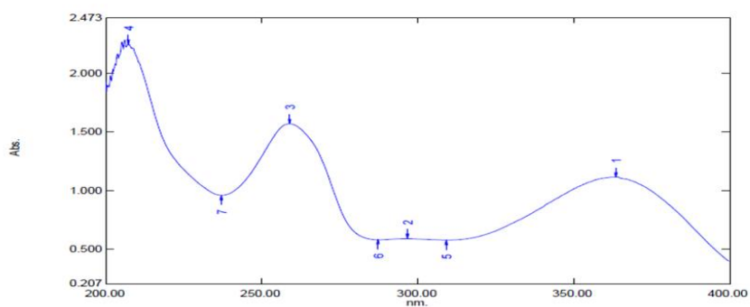
Fig. 1.2 UV spectrum standard rutin
