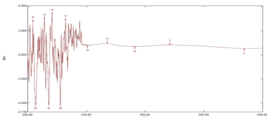
Fig. 1.5 UV spectrum ethyl acetate extract
