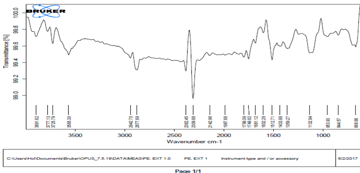
Fig. 2.3 FTIR spectrum of petroleum ether extract
