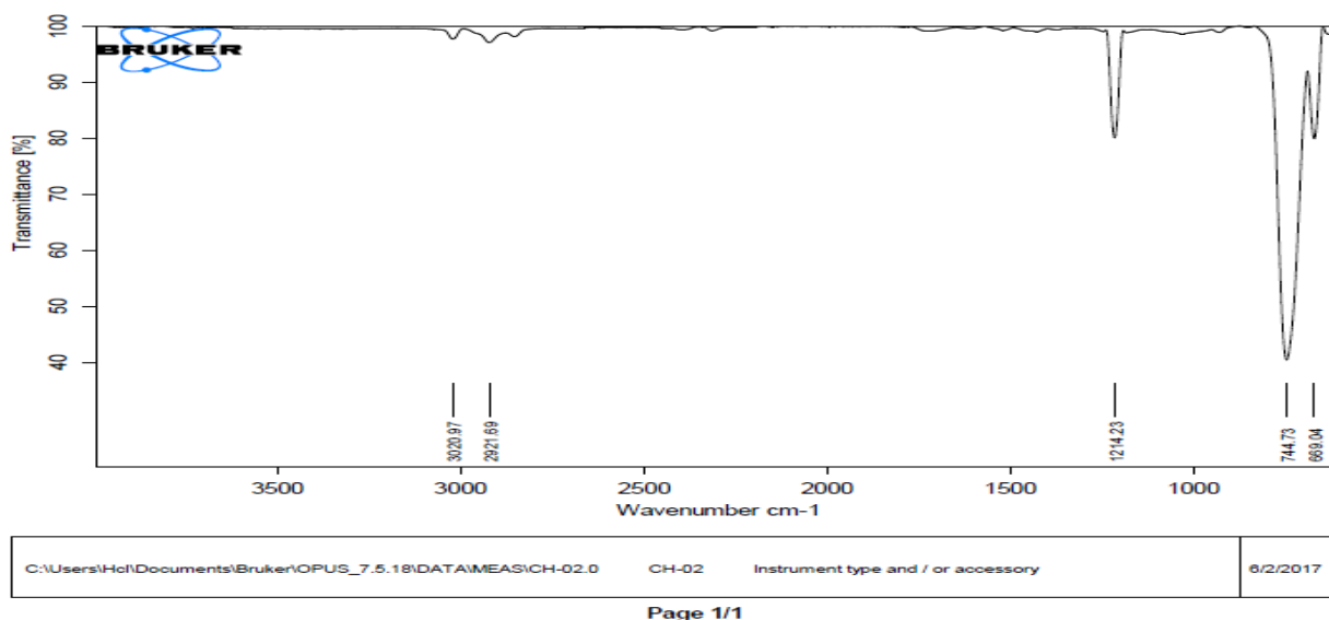
Fig. 2.4 FTIR spectrum of chloroform extract
