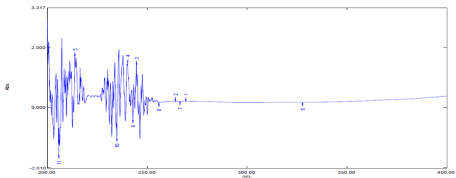
Fig. 1.3 UV spectrum petroleum ether extract
