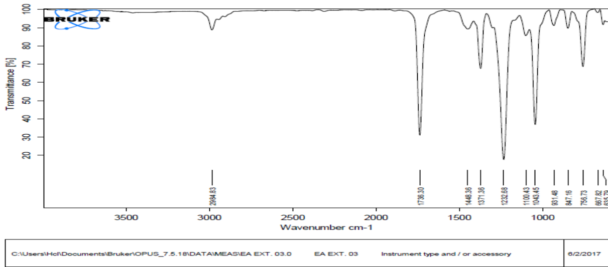
Fig. 2.5 FTIR spectrum of ethyl acetate extract
