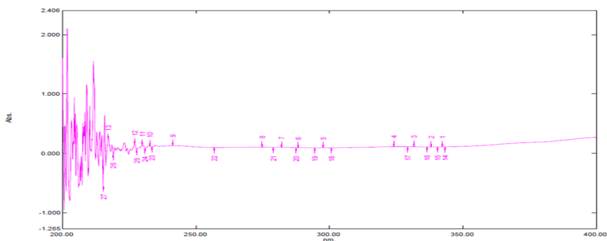
Fig. 1.4 UV spectrum chloroform extract
