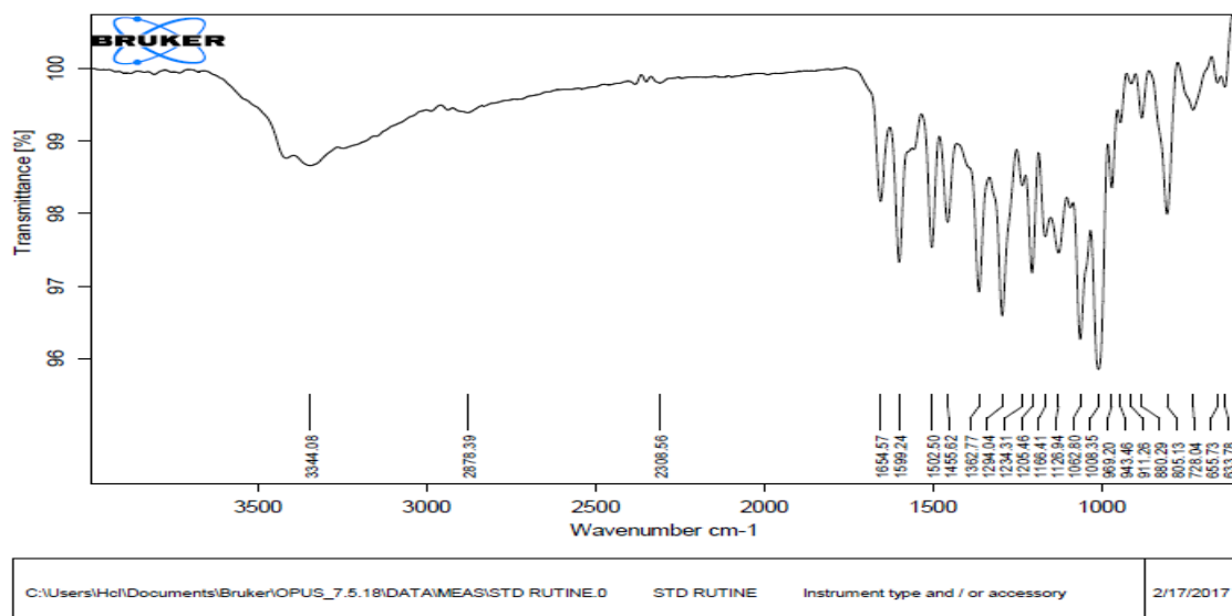
Fig. 2.2 FTIR spectrum of standard rutin
