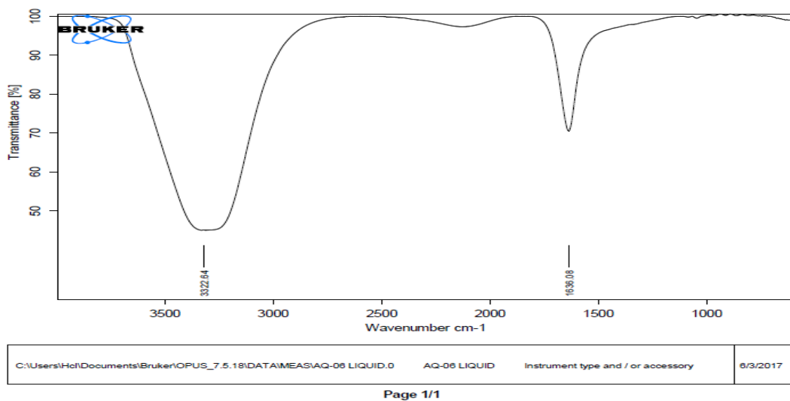
Fig. 2.7 FTIR spectrum of aqueous extract
