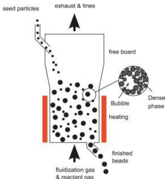
Figure 4: Fluidized-bed method
