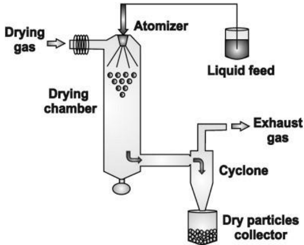
Figure 3: Spray drying method
