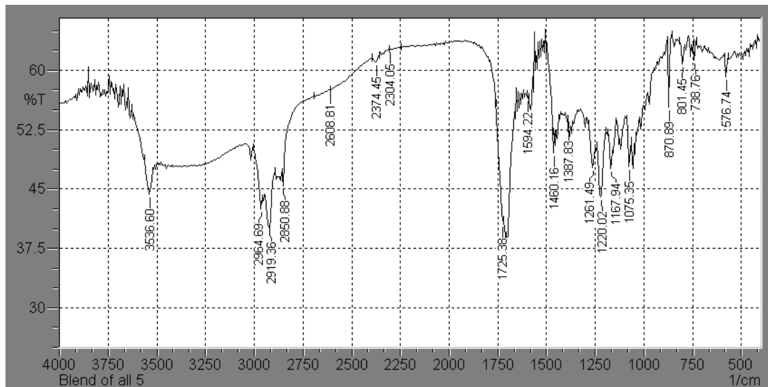
Figure 1(e): FTIR Spectrum of formulation blend
