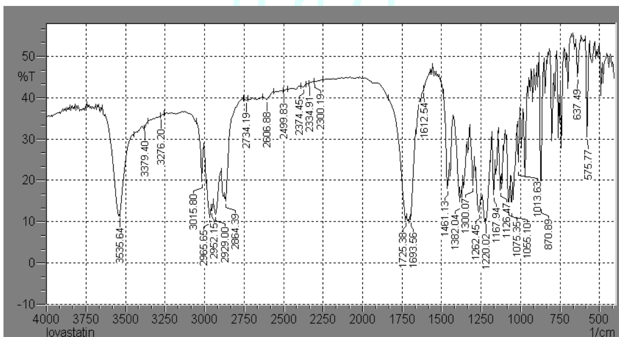
Figure 1(a): FTIR Spectrum of Lovastatin
