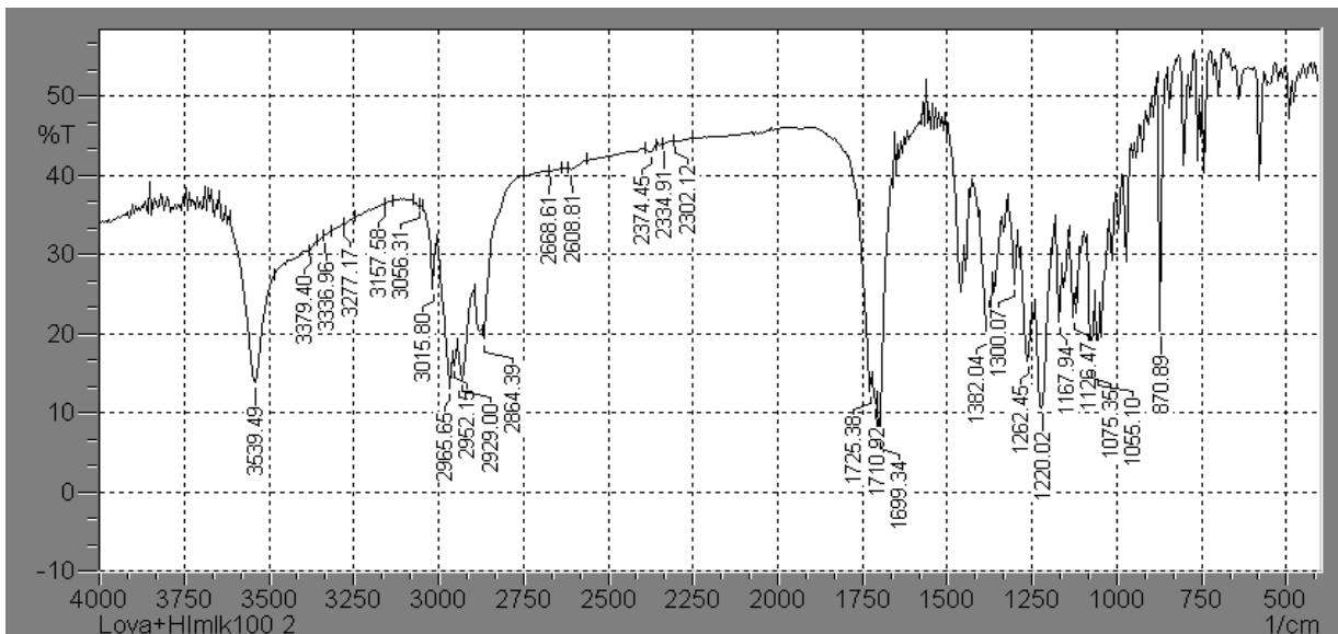
Figure 1(d): FTIR Spectrum of physical mixture of Lovastatin and HPMC K100M
