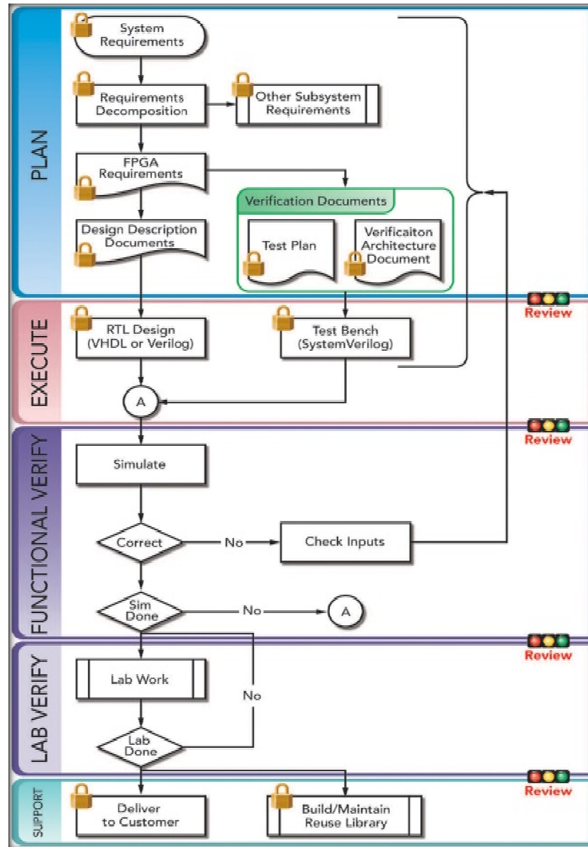
Figure 2. Typical Best Practice Electronic Design Process [11]
