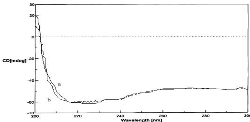
Figure 3: CD- Spectra of (a) Insulin from conjugated Nanoparticles, (b) Insulin.
