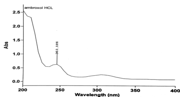
Figure 2: \lambda_{\text{Max}} of ambroxol hydrochloride
