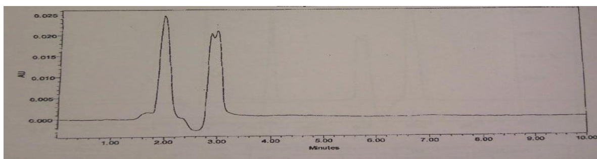
Figure 2: Blank Chromatogram
