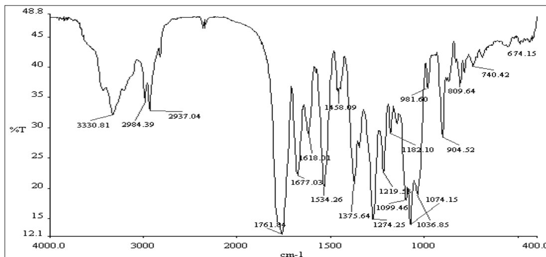
Figure 1: FTIR spectrum of cefuroxime axetil
