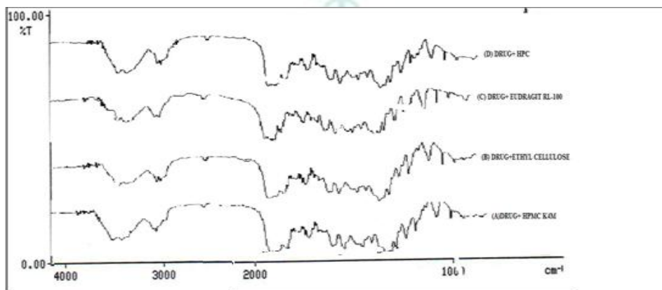
Figure 5: Comparative study of drug and excipients by FTIR spectrum (A) Drug+HPMC K4M (B) Drug+ethyl cellulose (C) Drug+Eudragit RL-100 (D) Drug+HPC
