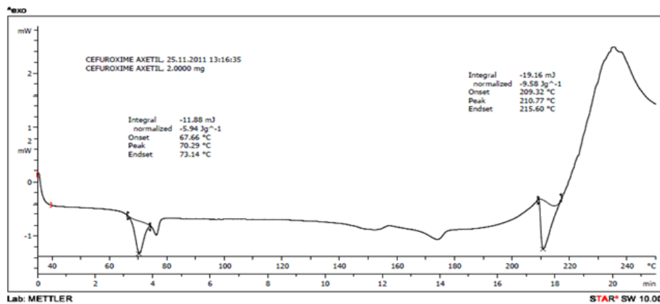
Figure 4: DSC graph of cefuroxime axetil
