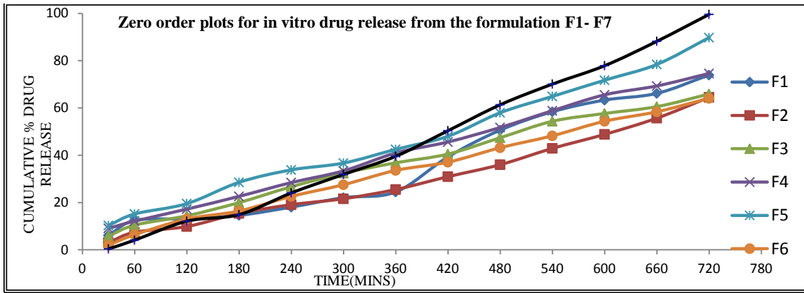
Figure 8: Zero order plots of the in vitro drug release from the formulations F1-F7
