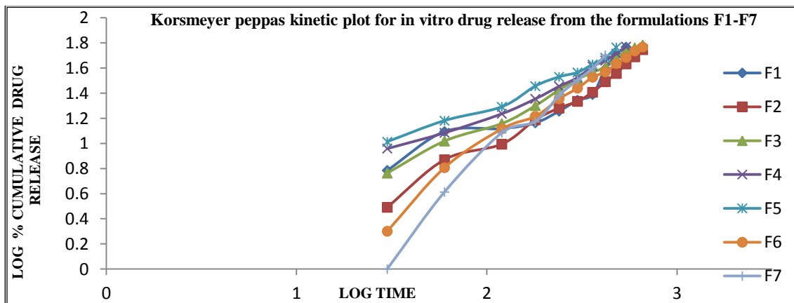
Figure 11: Korsmeyers peppas plots of the in vitro drug release from the formulations F1-F7
