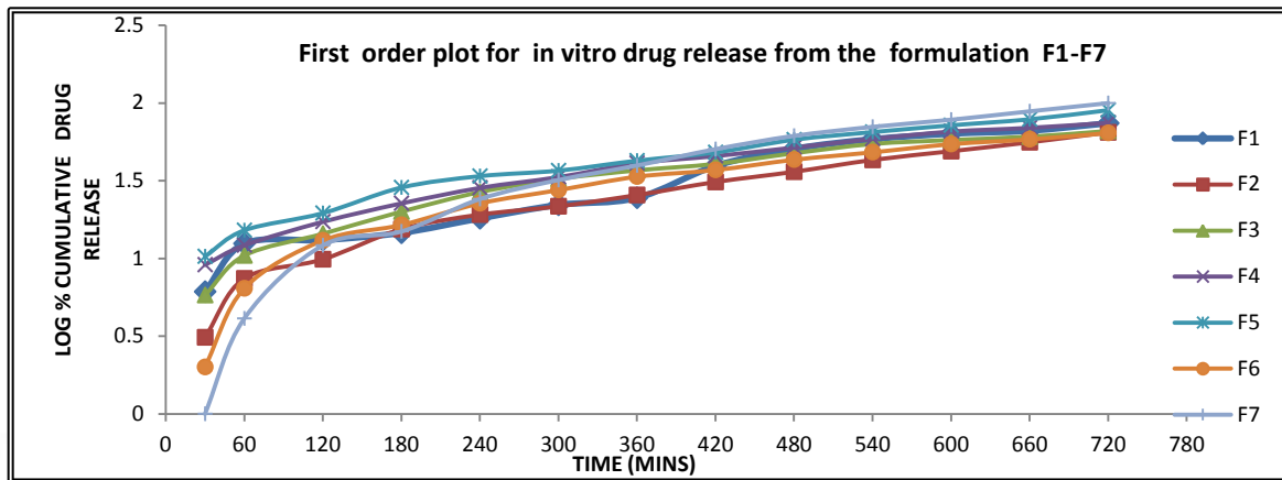
Figure 9: First order plots of the in vitro drug release from the formulations F1-F7
