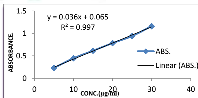
Figure 3: Calibration curve for cefuroxime axetil
