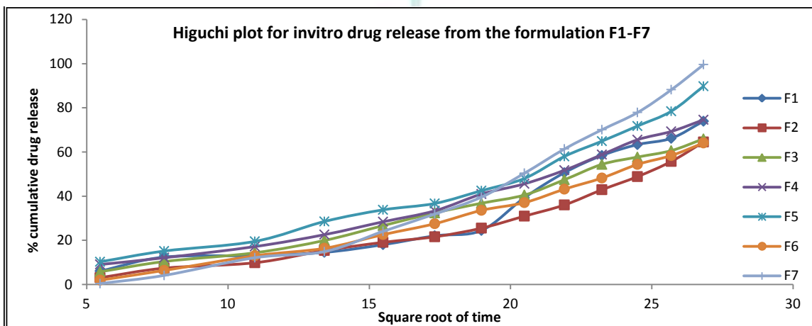
Figure 10: Higuchi plots of the in vitro drug release from the formulations F1-F7
