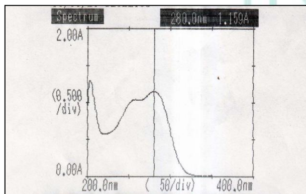
Figure 2: UV spectrum of Cefuroxime Axetil
