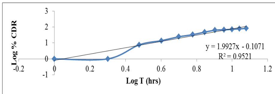
Figure 8: Korsmeyer Peppas model of enteric coated mucoadhesive tablet containing bael gum (F4)
