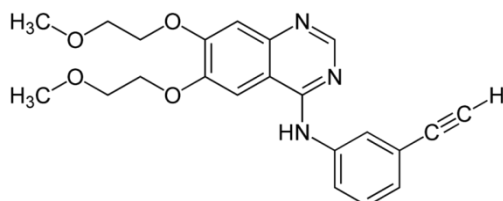
Figure 1: Structure of Erlotinib Hydrochloride
