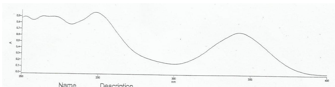
Figure 2: UV – Spectrum of Erlotinib Hydrochloride
