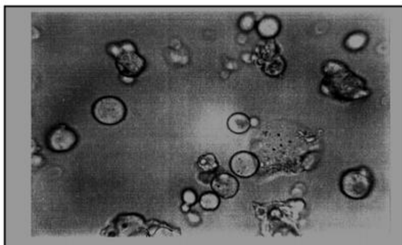
Figure 2: Optical micrograph of BSA-propranolol hydrochloride microspheres stabilized by heat denaturation method with an average size range of 1-25 \mu\text{m} , taken by a camera mounted light microscope (x1600). As it indicates microspheres have spherical shape.
