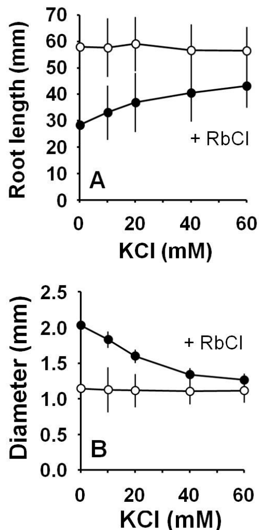
Figure 4 - Restoration of 20 mM RbCl-affected root growth of 2-d-old plants by KCl. Effects of KCl gradient on root length (A) and diameter (B) are shown. Vertical bars indicate standard deviations.
