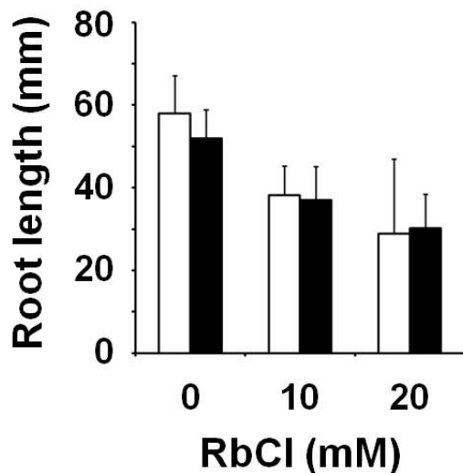
Figure 3 - RbCl-inhibited root growth after 2 d in the absence (white columns) and presence (black columns) of 4 mM silver thiosulfate (STS), an ethylene action inhibitor. STS was applied to the growth medium. Vertical bars indicate standard deviations.
