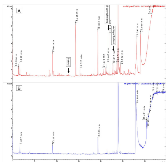
Figure 2 - GC/MS chromatograms of two different samples bc318 (A) and pr37h24 (B) as a representative of European and American genotypes.
