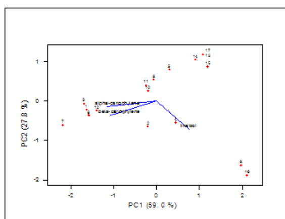
Figure 3 - Projection of 17 ND samples including European (1-12) and American genotypes (13-17) represented by three variables ( \alpha -caryophyllene, \beta -caryophyllene and linalool concentrations) onto the plot defined by the first and the second principal component. The outliers are genotypes Saxxoo (6) and A292 (16).
