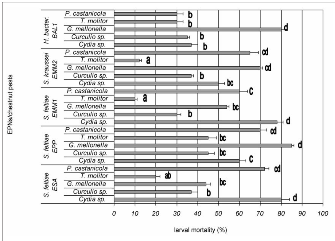
Fig. III – Mortality of chestnut pests' larvae infested 10 days after the treatment with 5 species and strains of EPNs. Columns marked with the same letter are not statistically different at p < 0.05 , according to the Turkey's HSD test.
