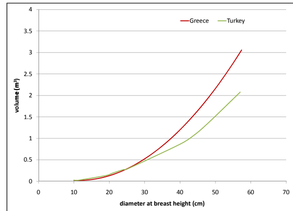
Figure 4 - Comparison of the two volume curves for Pinus brutia from Greece and Turkey.
