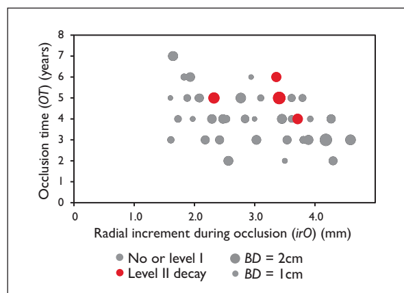
Figure 4 - Occlusion time ( OT ) as a function of radial increment during occlusion ( irO ) (n=63). Size of the markers corresponds to branch diameter ( BD ), size of data points are proportional to branch diameter. Level II decay is indicated in red.
