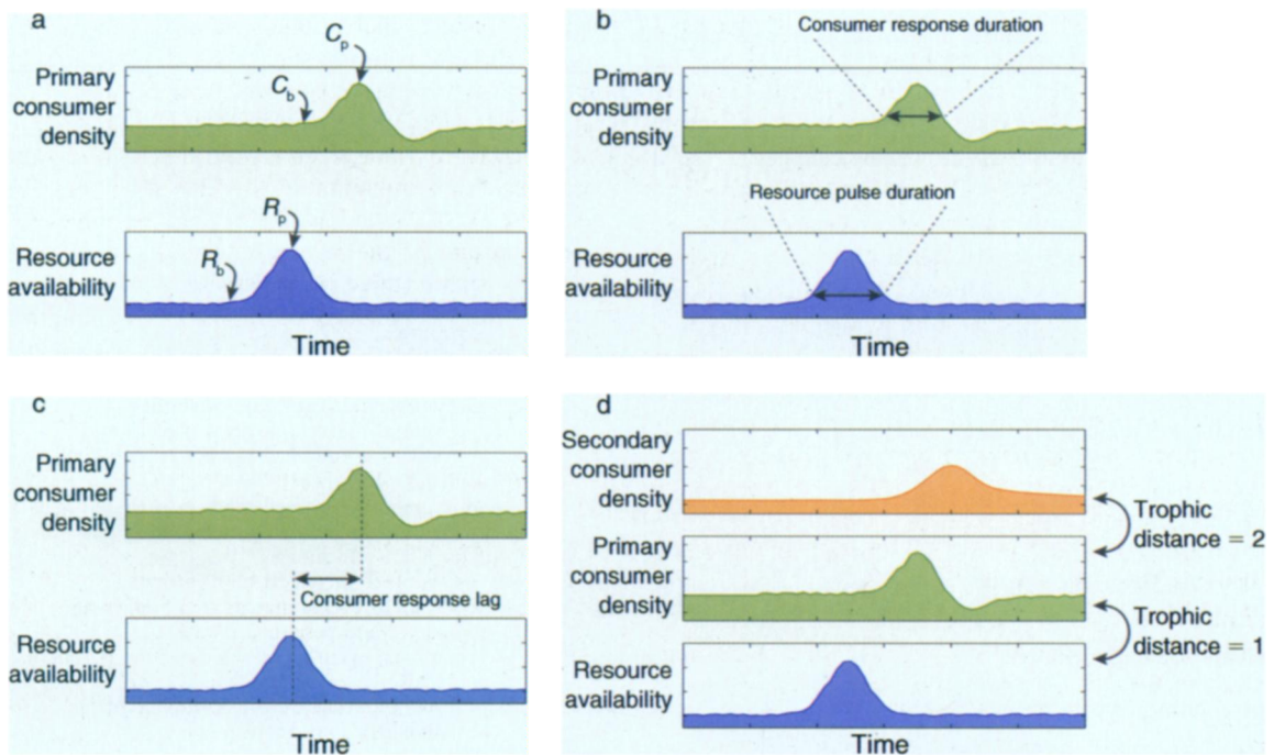
FIG. 1. A schematic diagram of extracted data used to investigate (a) resource pulse ( R_p ) and consumer response ( C_p ) magnitude relative to baselines ( R_b and C_b ), (b) resource pulse and consumer response duration, (c) the consumer response lag, and (d) indirect effects and trophic distance.
