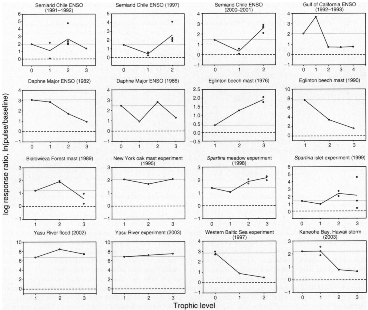
FIG. 8. The attenuation and amplification of indirect effects of 16 specific resource pulse events in 10 systems (see Table 1). Note that the y-axes represent log response ratios. The leftmost point in each panel represents the resource pulse magnitude for the primary resource pulse(s); all other points represent consumer response magnitudes. A solid line connects the mean response magnitude for each trophic level; a positive slope line leading to a trophic level indicates an amplifying response, while a negative slope line indicates an attenuating response. The solid gray line in each panel represents the magnitude of the primary resource pulse; response ratios above this line indicate consumer responses larger than the primary resource pulse, reflecting amplification relative to the initial resource pulse. By comparison, response ratios below this line represent response ratios smaller than the initial resource pulse, reflecting attenuation relative to the initial resource pulse. The dashed line in each panel represents the zero threshold; the height of response ratios above this line indicates the magnitude of positive responses relative to their baseline conditions. The abbreviation “ENSO” stands for El Niño Southern Oscillation.
