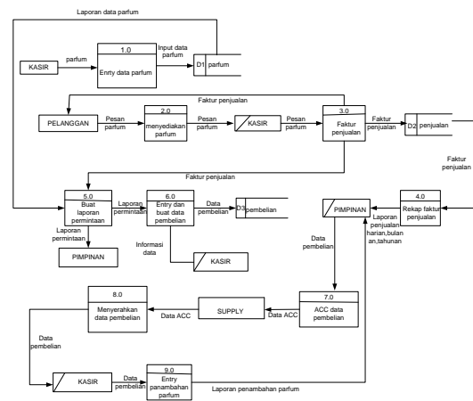
Gambar 3.7 Data Flow Diagram
