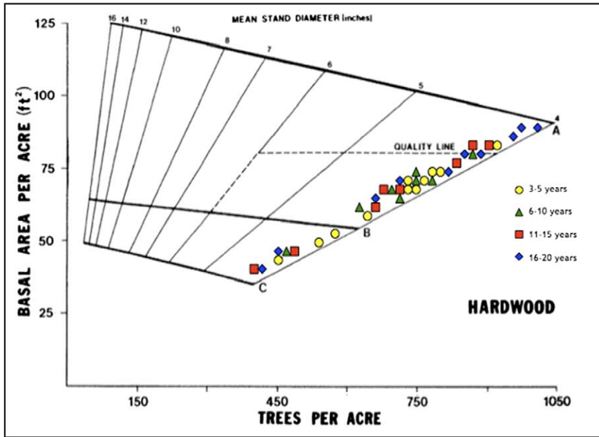
Fig. 4. Stocking guide for main crown canopy of even-aged hardwood and mixed-wood stands relative to basal area, number of trees per acre, and mean stand diameter. The A-line is fully stocked, the B-line is suggested residual stocking (~60%), and the C-line is minimum stocking (~40%) (Leak et al. 1987). The proportion (%) of commercial trees without severe damage are plotted by age class; stocking is projected to a 4" mean stand diameter.
