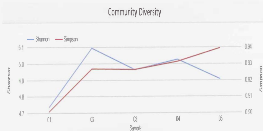
Figure 18: Differences in bacterial diversity within tick samples
