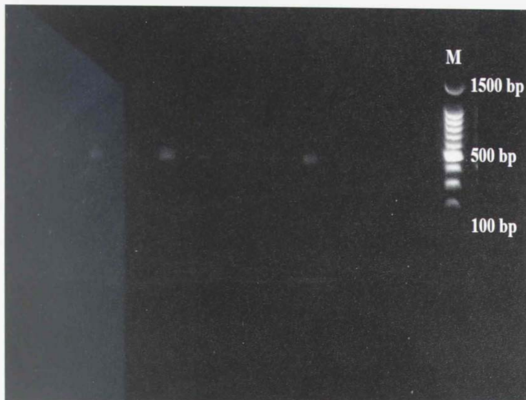
Figure 35: Agarose gel electrophoresis of PCR products of O. muesebecki samples with Tm16S+1/ Tm16S-1 primer set
