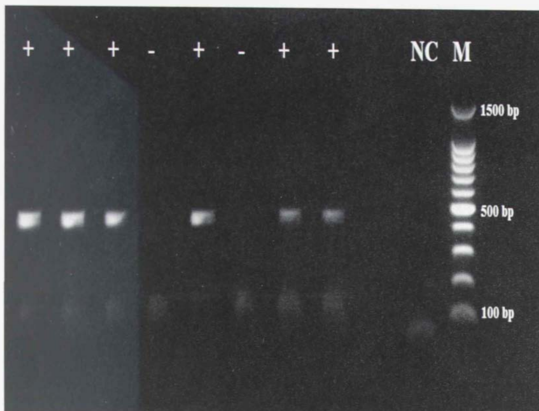
Figure 34: Agarose gel electrophoresis of PCR products of O. muesebecki samples with 16S+1/16S-1 primer set
