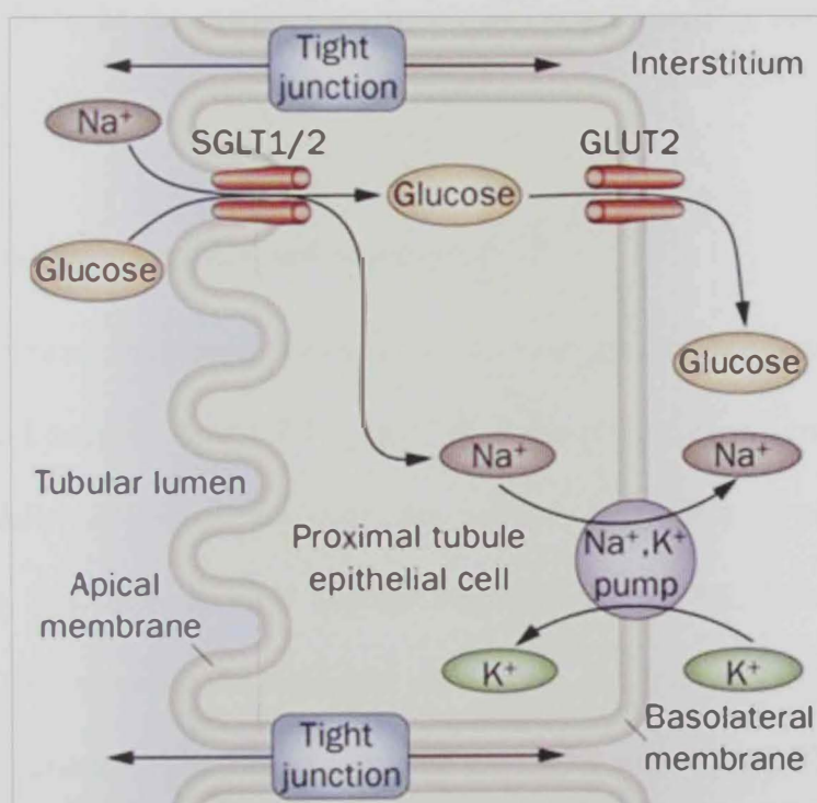
Figure 1-20: Mechanism of glucose transport by sodium/glucose co-transporters
