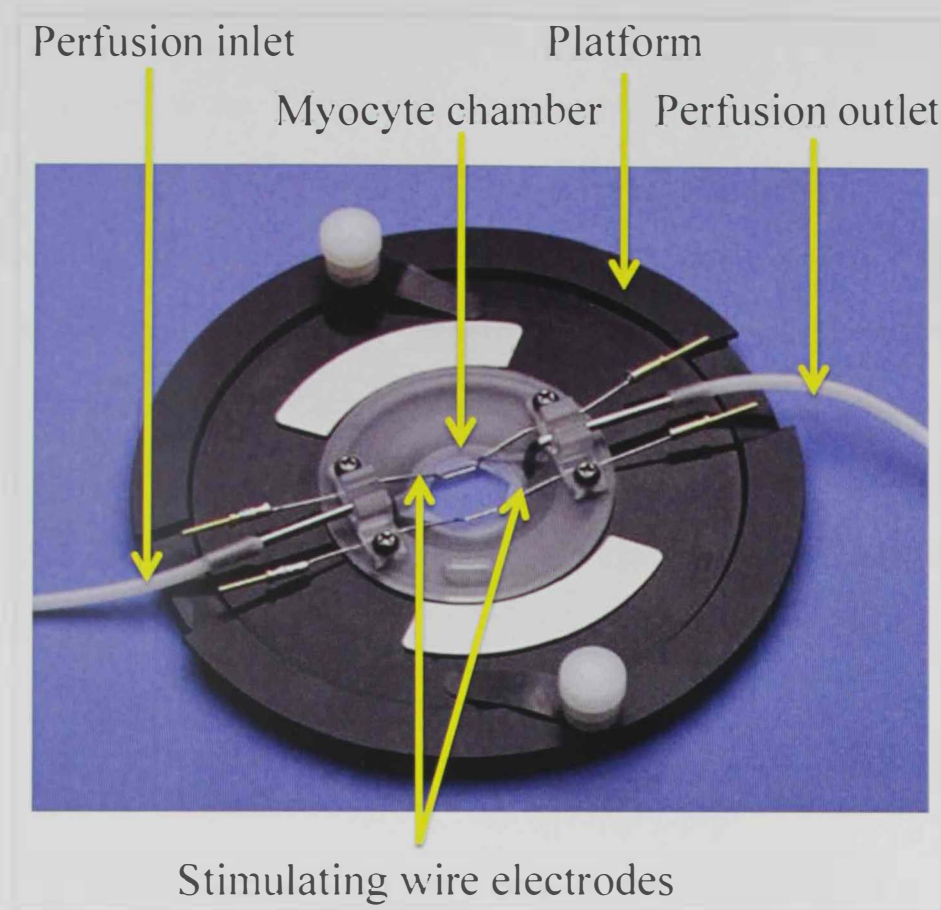
Figure 3-9: Myocyte perfusion chamber with field stimulation
