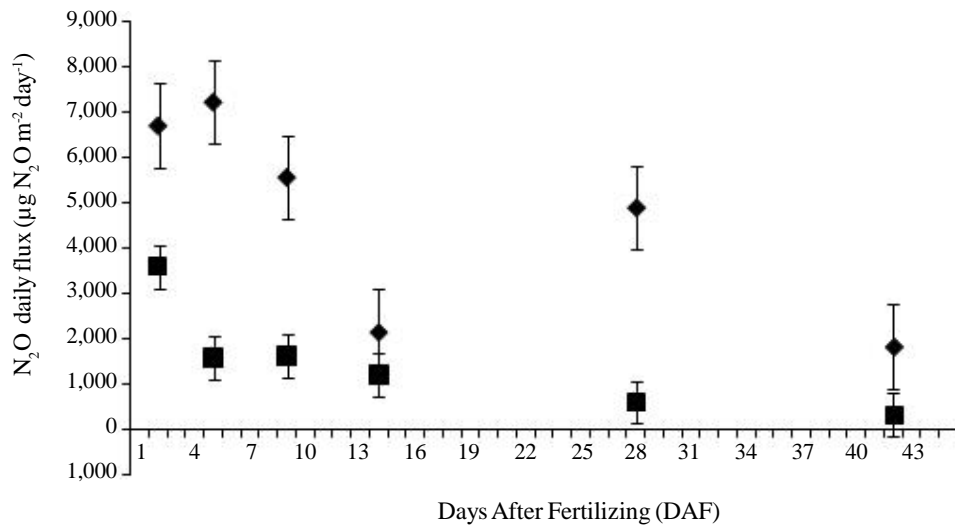
Figure 3. Daily N 2 O emission from maize site. —◆—: vertisol, —■—: inceptisol.
