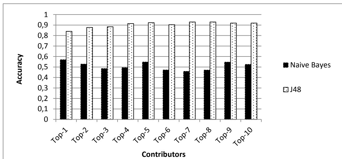
Figure 3. Accuracy: Naïve Bayes versus J48
