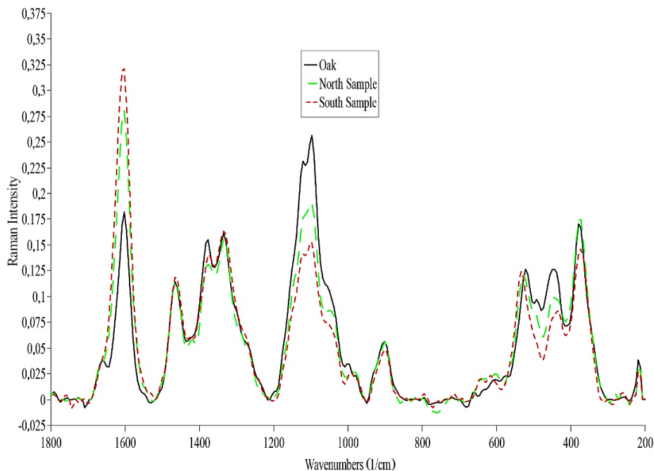
Figure 4: FT-Raman for historical and fresh sample of oak.
