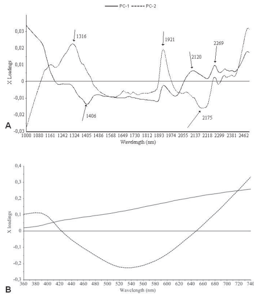
Figure 5: X-loadings of NIR spectra (a) pretreated with MSC and (b) visible spectra
