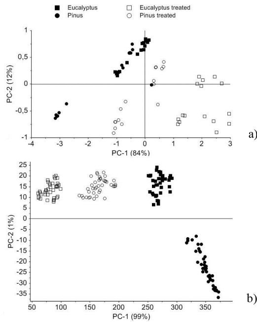
Figure 4: Principal component analysis of (a) NIR spectra and (b) visible spectra (B).
