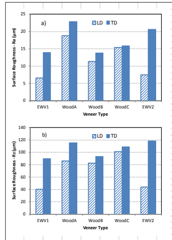
Figure 5. Comparison of surface roughness data from various veneers with finger joint region for Wood A , Wood B and Wood C . ENV1 and ENV2 are engineered wood veneers from Triplochiton scleroxylon and Tilia amurensis , respectively. a) Ra and b) Rz.
