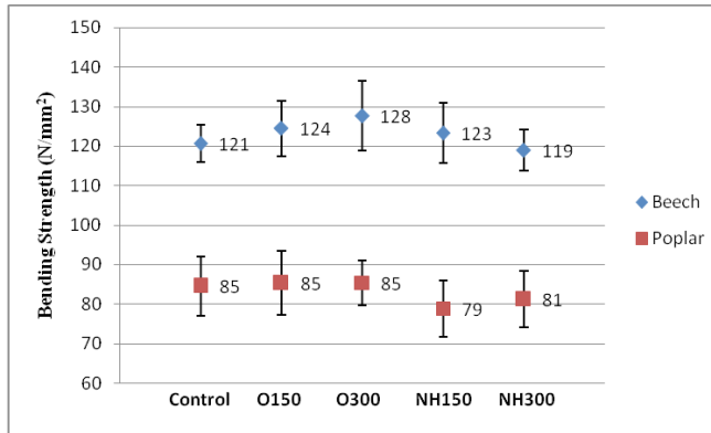
Figure 2. Bending strength (MOR) of the test panels.
