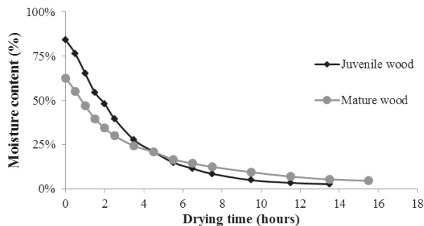
Figure 2. Drying curve with average moisture content and drying time values for samples of 37-year-old Eucalyptus saligna wood.
