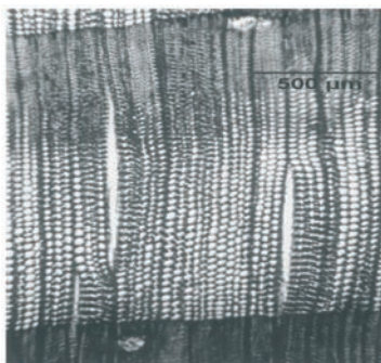
Fig. 3a+b. Liquid full hydro thermolysed treated Scots pine (cross section), radial cracks in the earlywood
