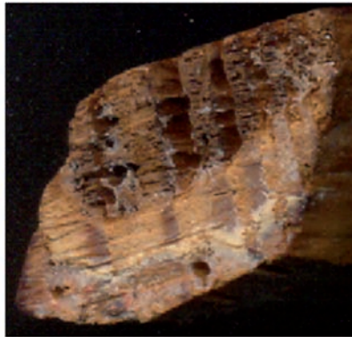
Figure 4. Details of degradation by Gloeophyllum sepiarium on non-impregnated pinewood ( T_0 ).
