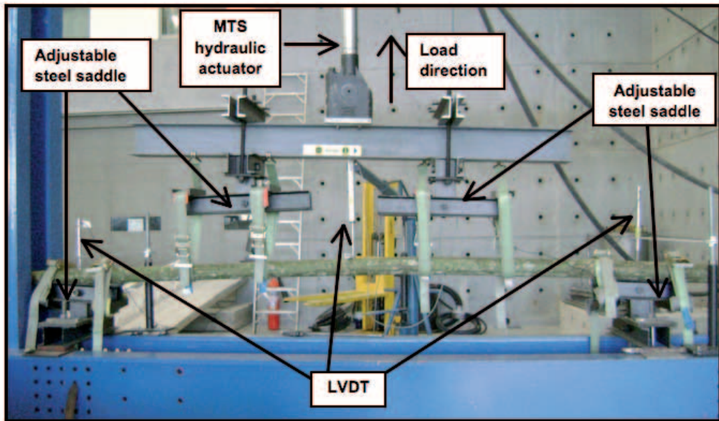
Figure 4. Bending test setup
