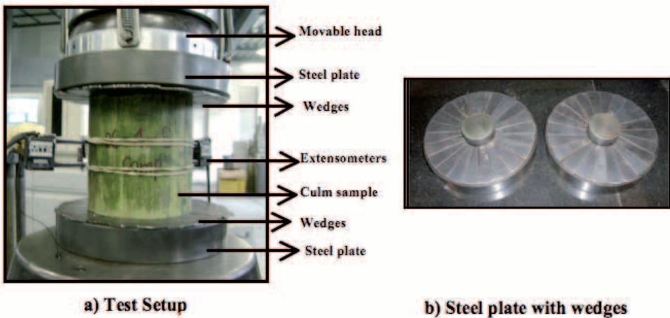
Figure 2. Compressive test setup and steel plates
