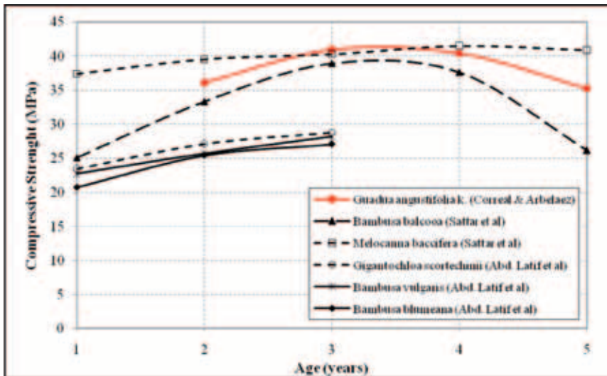
Figure 5. Variation of compressive strength for different bamboo species with age
