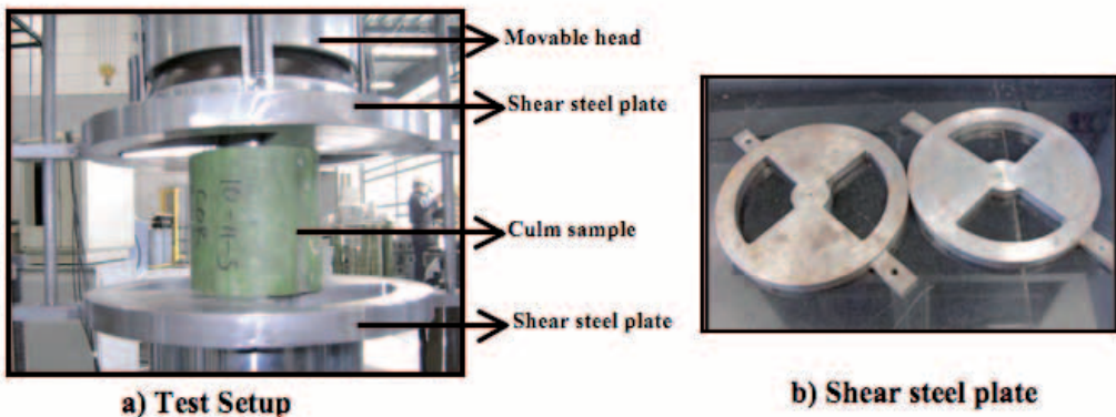
Figure 3. Shear test setup and steel plates
