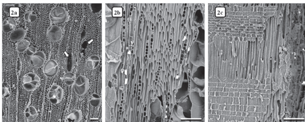
Figure 2. Plate 2. Corymbia maculata . Charcoal micrographs. Arrows show the ruptures. Sections (a) Transverse, (b) Tangential Longitudinal, (c) Radial Longitudinal. Bars: 100 \mu m.
