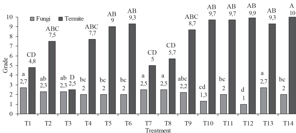
Figure 2. Average deterioration rates, assigned on the basis of the analysis of the occurrence and action of fungi and termites in wood thermorectified Eucalyptus grandis , exposed in the test field after ten months.
