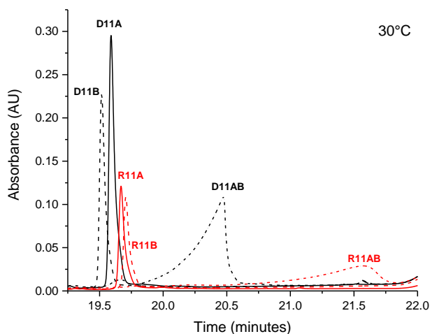
Figure 2: IP RP UHPLC Analysis of the 11mer oligonucleotides. The samples were analyzed on a BEH C18 column at 30°C using Gradient 1.
