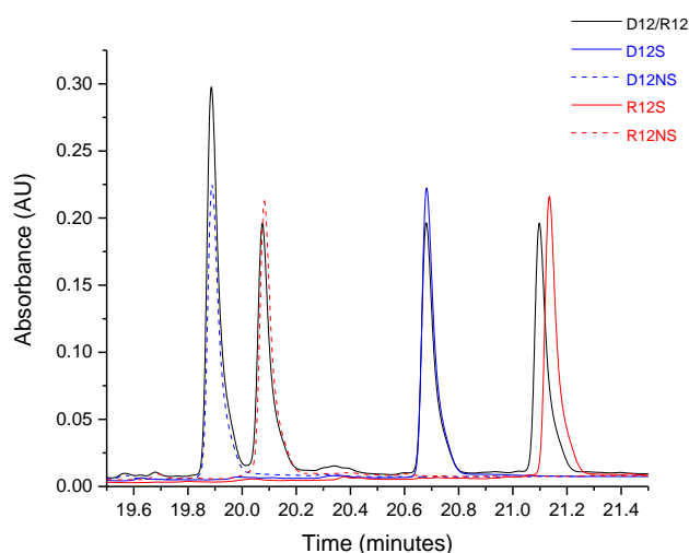
Figure 6: IP RP UHPLC analysis of the 12mer DNA/RNA mixture, 12mer DNA, and 12mer RNA using Gradient 1 at 30°C. The chromatogram is an overlay of the 12mer DNA/RNA mixture with the D12 and R12 oligonucleotides.
