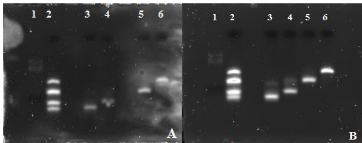
Figure 7: PAGE of 12mer DNA and RNA oligonucleotides. Lane 1 contains microRNA marker, Lane 2 contains D12/R12 mixture, Lane 3 contains D12S, Lane 4 contains D12NS, Lane 5 contains R12S, and Lane 6 contains R12NS (A) 15% native PAGE analysis of 25.0 ng/μ D12/R12 mixture and 12.5 ng/μl 12mer DNA and 12mer RNA. (B) 15% native PAGE analysis of 12mer 25.0 ng/μl D12/R12 mixture, 12mer DNA, and 12mer RNA.
