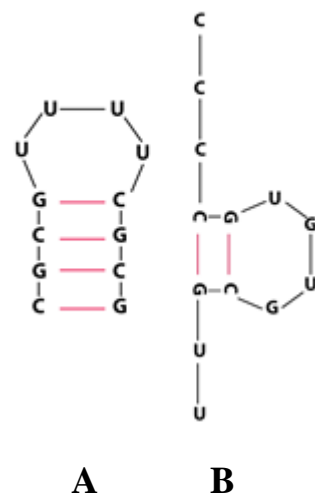
Figure 4: Structure of 12mer RNA oligonucleotide. A) Structure of the 4 base-pair tetraloop oligonucleotide (R12S) B) Structure of the 2 base-pair tetraloop oligonucleotide (R12NS)
