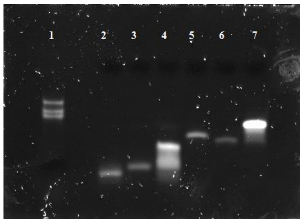
Figure 3: 15%PAGE of 11mer DNA and RNA oligonucleotides. Lane 1 contains microRNA marker, Lane 2 contains D11A, Lane 3 contains D11B, Lane 4 contains D11AB, Lane 5 contains R11A, Lane 6 contains R11B, and Lane 7 contains R11AB
