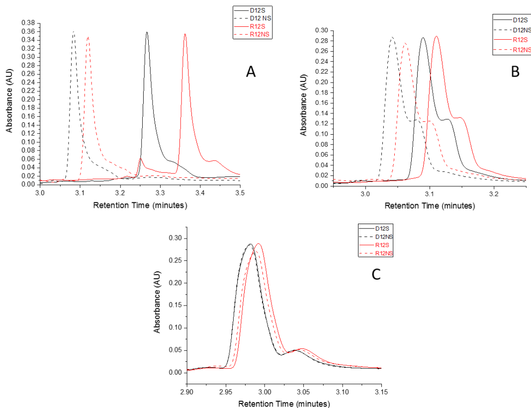
Figure 5: IP RP UHPLC analysis of 12mer DNA and RNA oligonucleotides. The samples were analyzed on a BEH C18 column at (A) 30°C, (B) 60°C, and (C) 80°C using Gradient 2.
