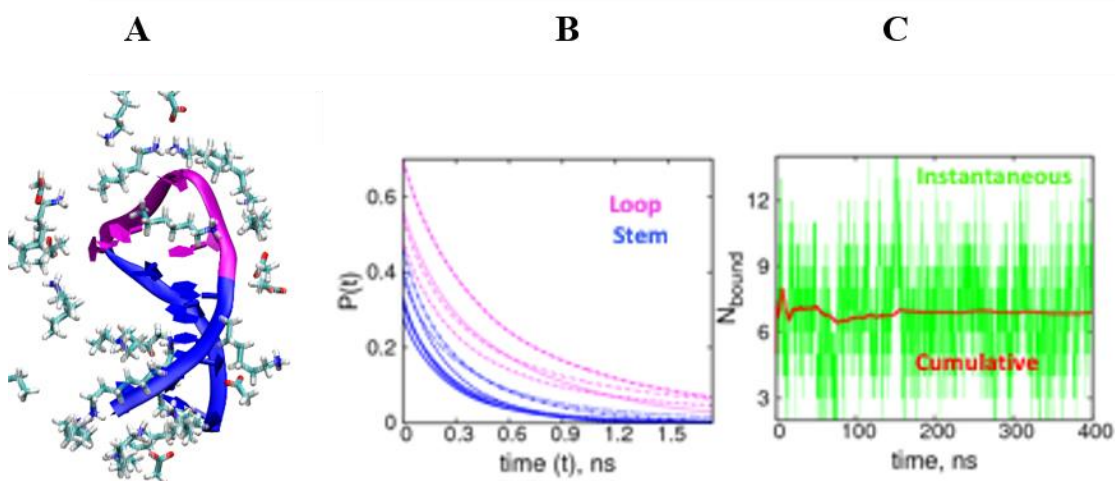
Figure 8: MD Simulation of R12S oligonucleotide. A) Simulation of R12S oligonucleotide B) Nanoscale timescale stimulation of the probability of HAA binding to R12S stem and loop regions C) Plot of instantaneous and cumulative amount of HAA bound to the loop region of R12S
