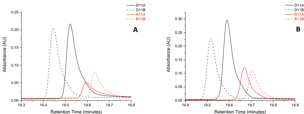
Figure 1: IP RP UHPLC analysis of 11mer DNA and RNA oligonucleotides. The samples were analyzed on a BEH C18 column at 30°C using Gradient 1. (A) Analysis of 11mer oligonucleotides before the addition of ammonium phosphate to buffer A and B. (B) Analysis of 11mer oligonucleotides after the addition of ammonium phosphate to buffer A and B.
